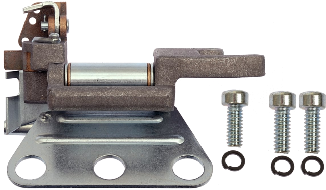
FRONT LIFTER ASSY COMPLETE. - C2 p/n 33397
