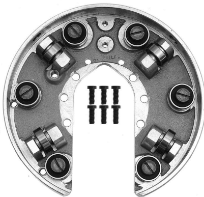
REAR PLATE ASSEMBLY - C2 p/n 27689
