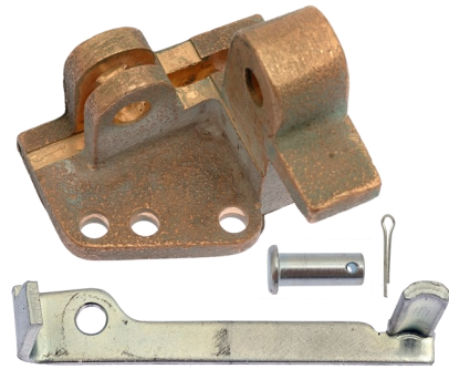
HINGE BRACKET KIT - C2 p/n 33400
